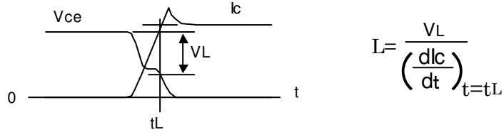
Fig. Difinition of stray inductance
