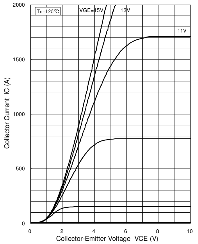
Collector Current vs. Collector to Emmitter Voltage
